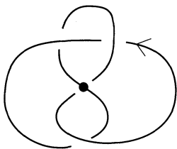
Figure 24. The knot 4_2 .
