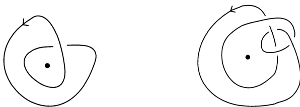
Figure 23. Quotient knots.
