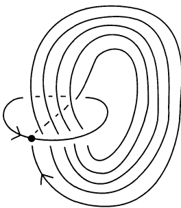
Figure 25. T_5 .
