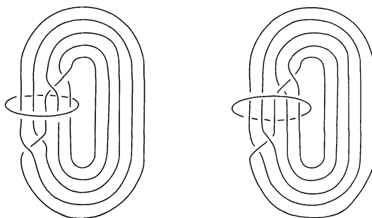
Figure 12. Amphicheiral link.
